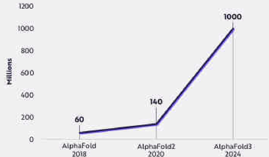
Structures Predicted
