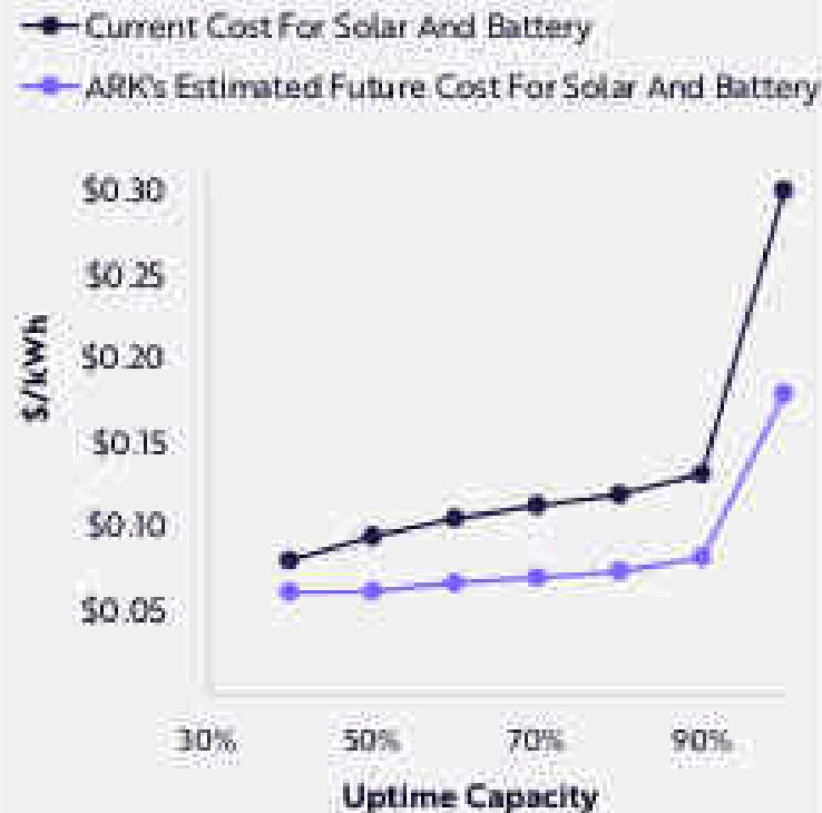
Lowest Levelized Cost Of Energy For Desired Uptime
