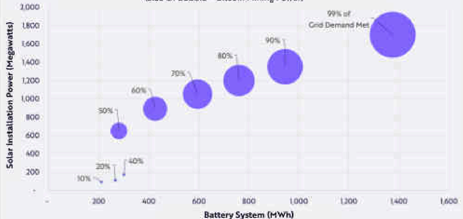
Solar, Battery, Bitcoin Systems Required To Meet Grid Dispatch Targets At Constant Cost Of Electricity
