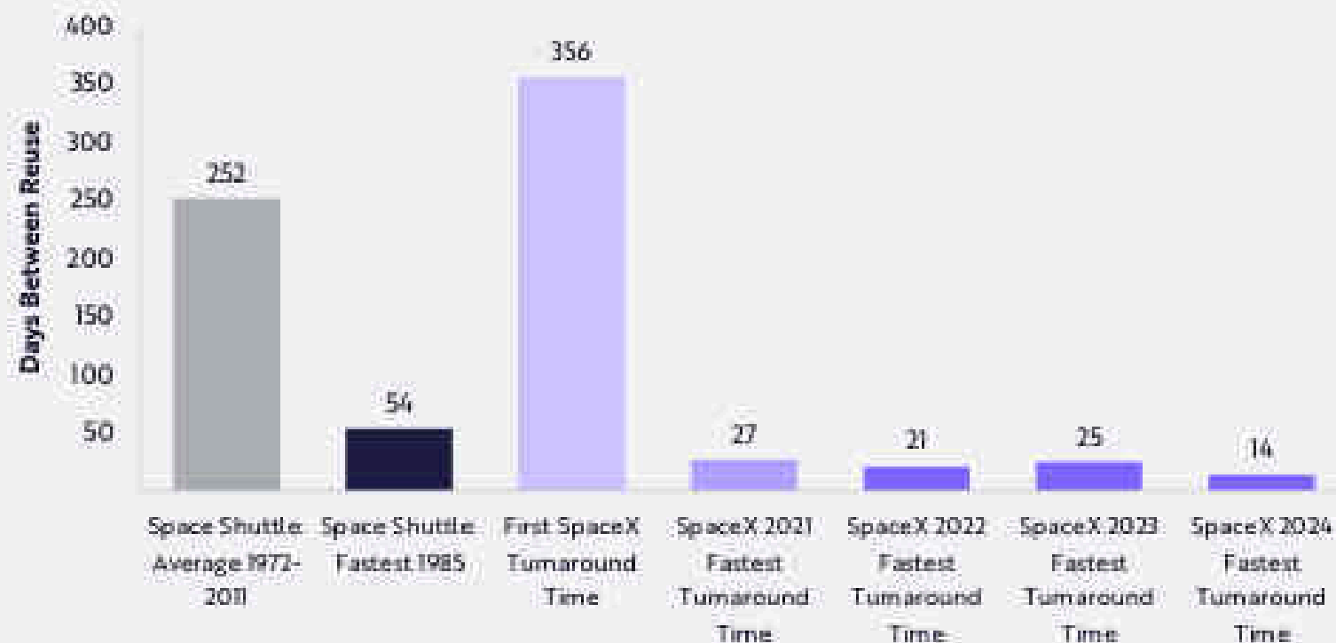
Rocket Turnaround Time
